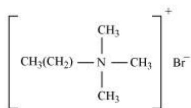
Cetyltrimethylammonium bromide
